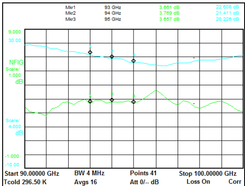
Figure 2: ERZ-LNA-9300-9500-20-4 Noise Figure
