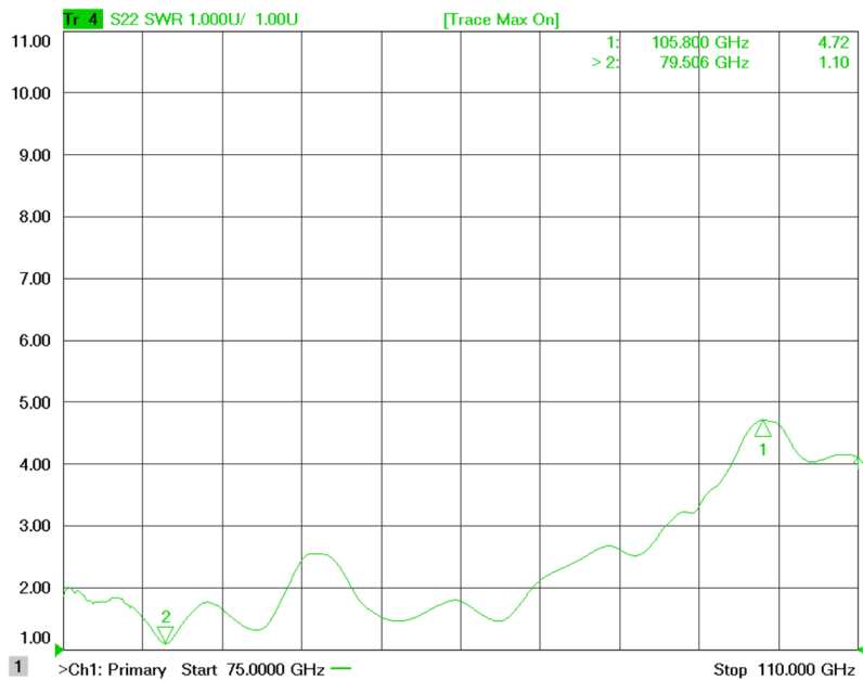
Figure 5: ERZ-LNA-7500-11000-20-4 S22
