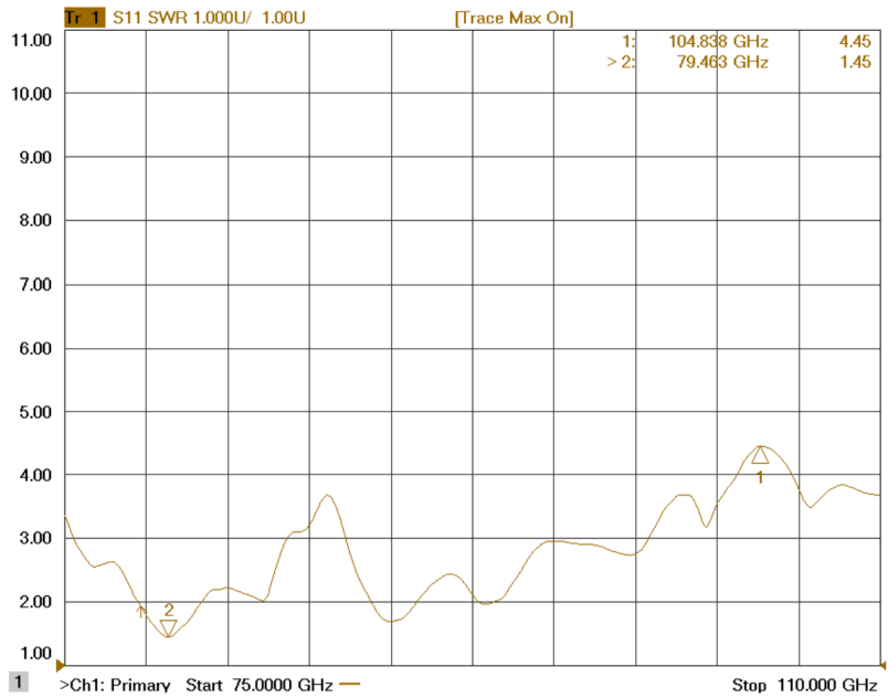
Figure 4: ERZ-LNA-7500-11000-20-4 S11
