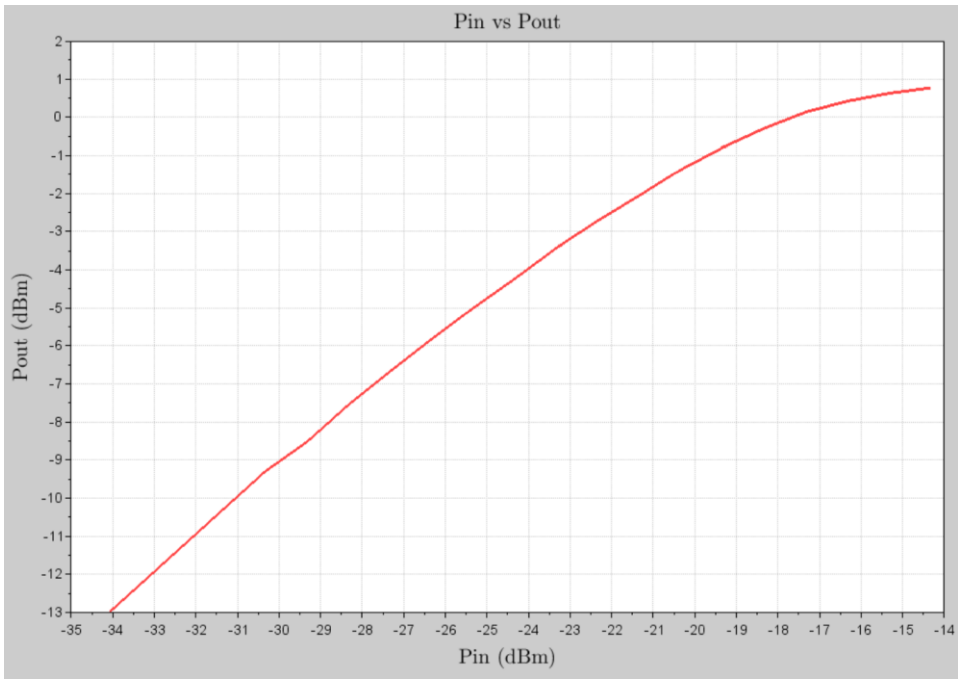
Figure 5: ERZ-LNA-7500-11000-20-4 Pout at 90 GHz
