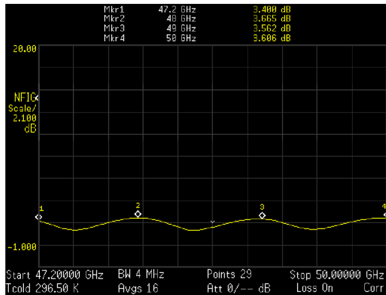
Figure 2: ERZ-LNA-4720-5140-15-4 Noise Figure
