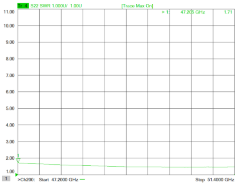
Figure 4: ERZ-LNA-4720-5140-15-4 Output Matching
