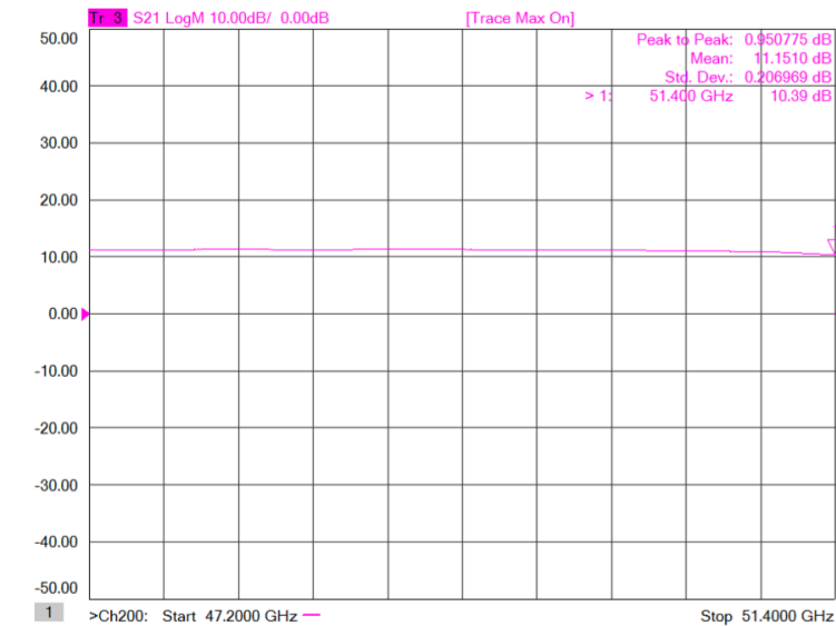
Figure 1: ERZ-LNA-4720-5140-15-4 Small Signal Gain
