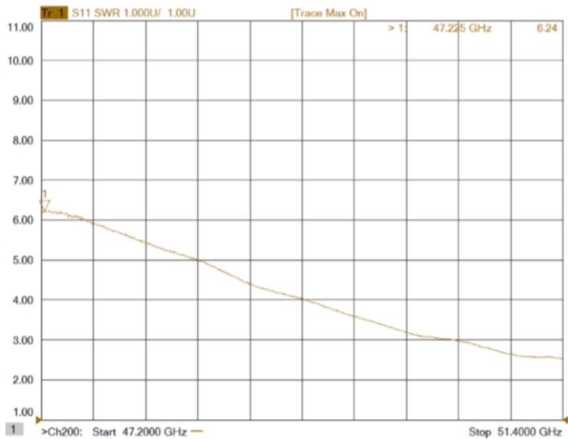
Figure 3: ERZ-LNA-4720-5140-15-4 Input Matching
