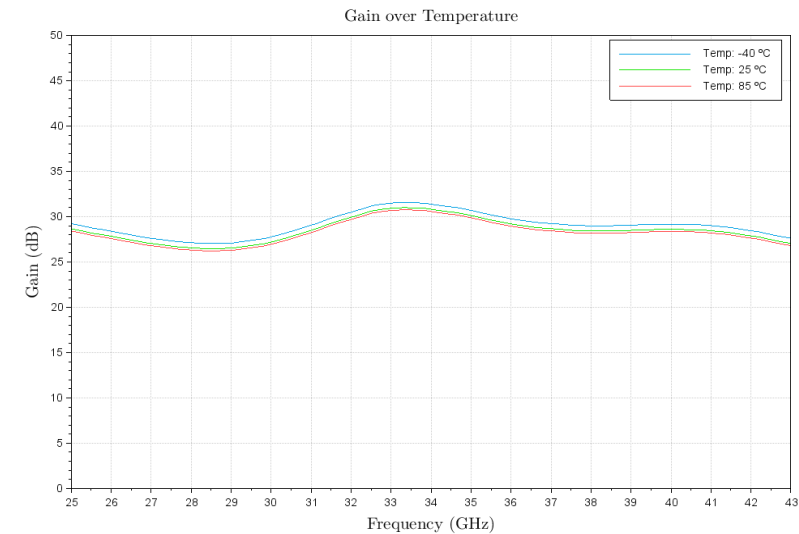
Figure 3: ERZ-LNA-2500-4300-33-2 Small Signal Gain Vs Temperature
