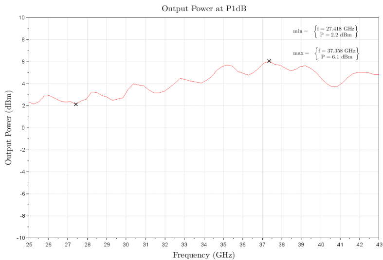
Figure 1: ERZ-LNA-2500-4300-33-2 P1dB
