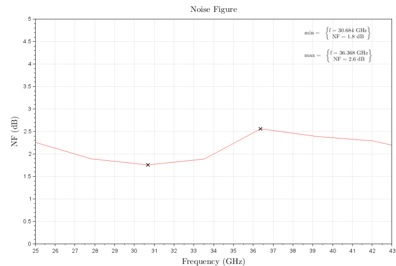
Figure 4: ERZ-LNA-2500-4300-33-2 Noise Figure
