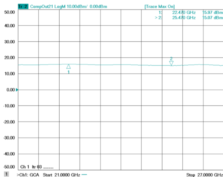
Figure 1: ERZ-LNA-2100-2700-25-2-NS P1dB
