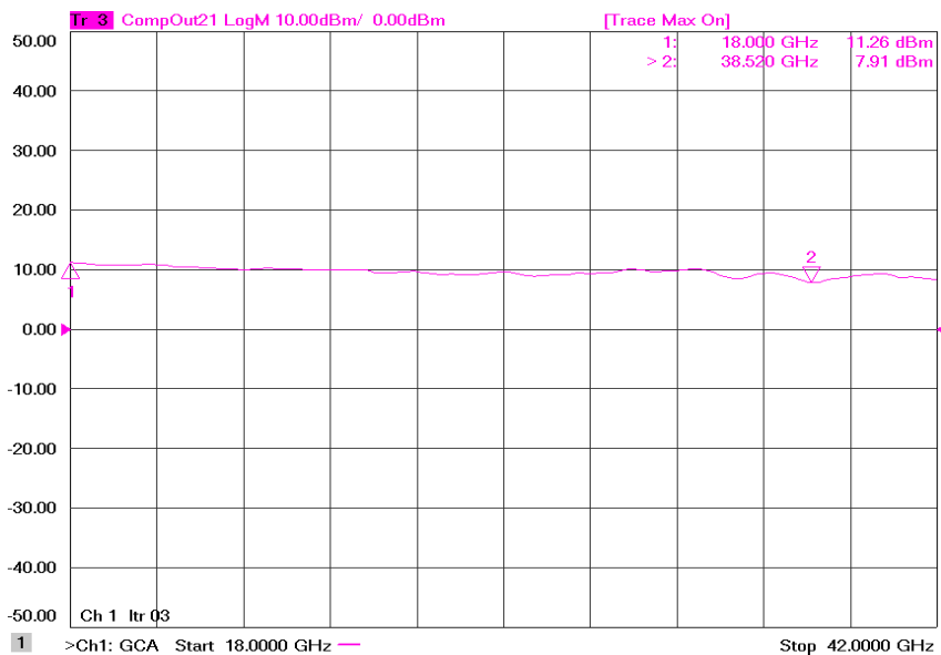
Figure 1: ERZ-LNA-1800-4200-24-6 P1dB
