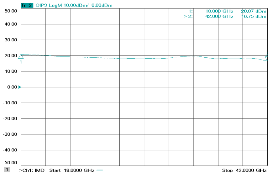
Figure 5: ERZ-LNA-1800-4200-24-6 OIP3
