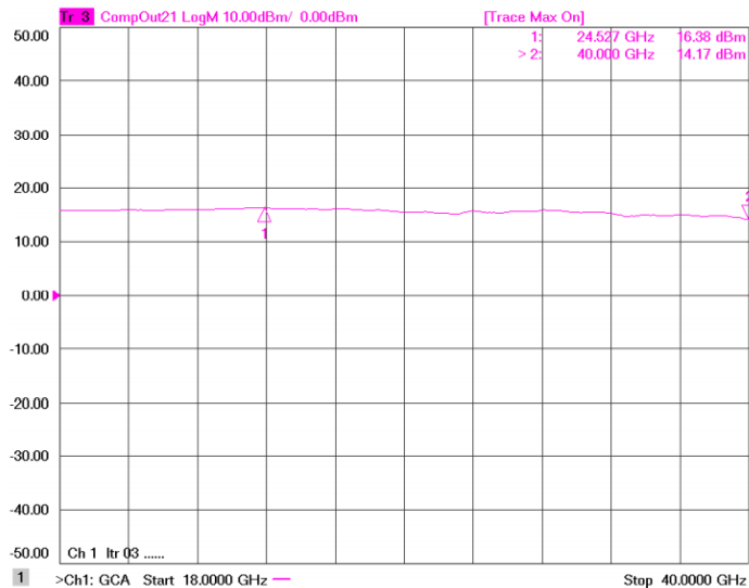
Figure 3: ERZ-LNA-1800-4000-23-12 P1dB
