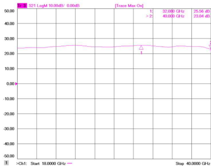
Figure 1: ERZ-LNA-1800-4000-23-12 Small Signal Gain at min att
