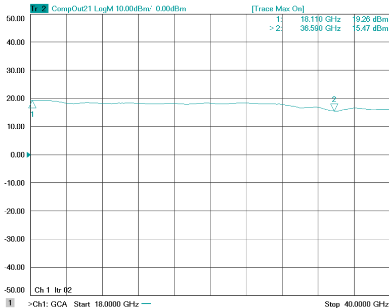
Figure 1: ERZ-LNA-1800-4000-15-4 P1dB
