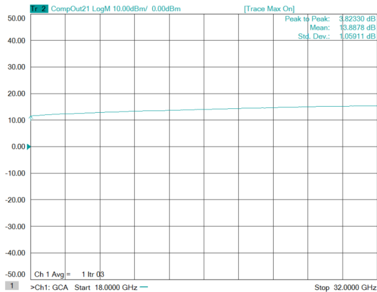
Figure 1: ERZ-LNA-1800-3200-21-3 Psat
