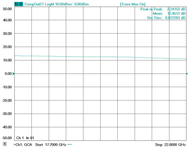
Figure 1: ERZ-LNA-1770-2200-70-2 P1dB
