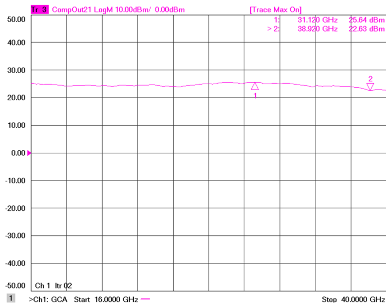
Figure 1: ERZ-LNA-1600-4000-28-6 P1dB
