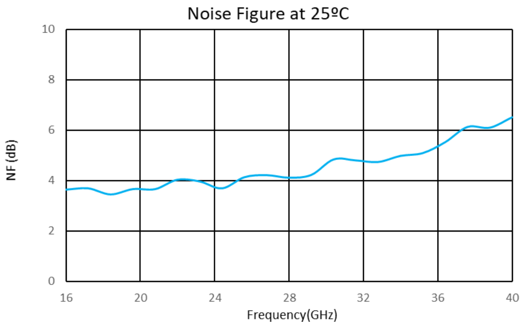
Figure 4: ERZ-LNA-1600-4000-28-6 Noise Figure
