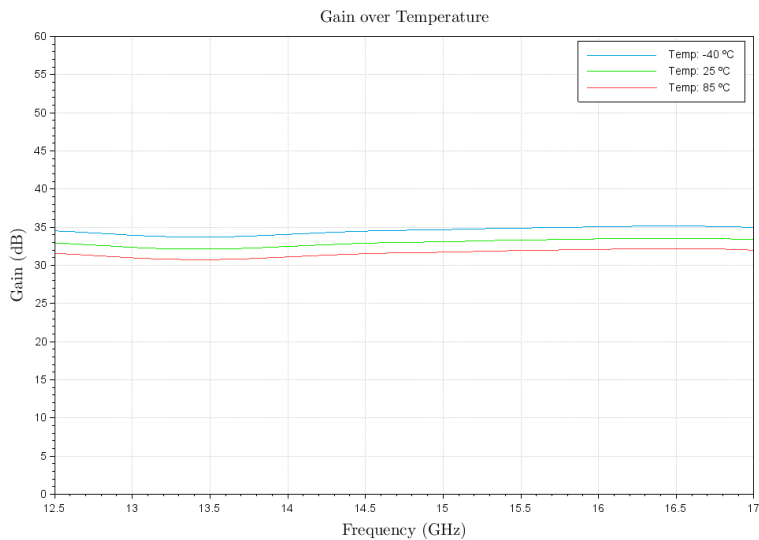
Figure 3: ERZ-LNA-1250-1700-33-3 Small Signal Gain Vs Temperature
