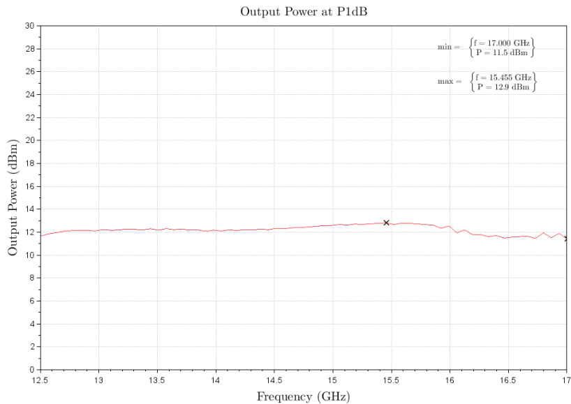
Figure 1: ERZ-LNA-1250-1700-33-3 P1dB
