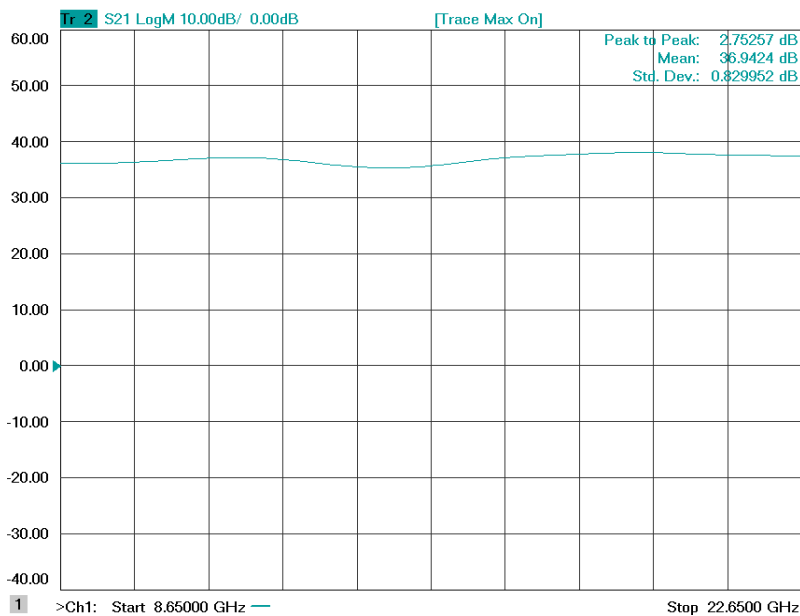
Figure 2: ERZ-LNA-0865-2265-30-3 Small Signal Gain
