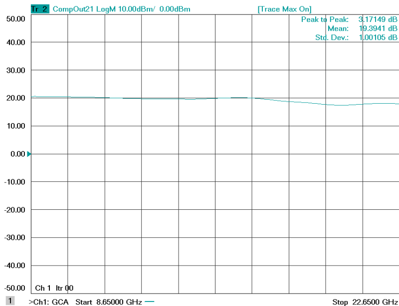
Figure 1: ERZ-LNA-0865-2265-30-3 P1dB
