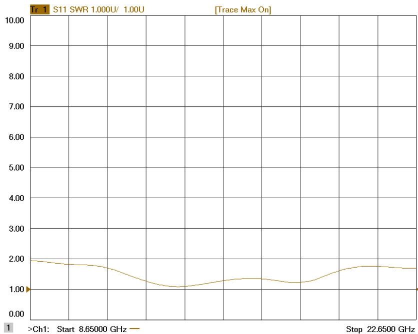
Figure 4: ERZ-LNA-0865-2265-30-3 Input Matching
