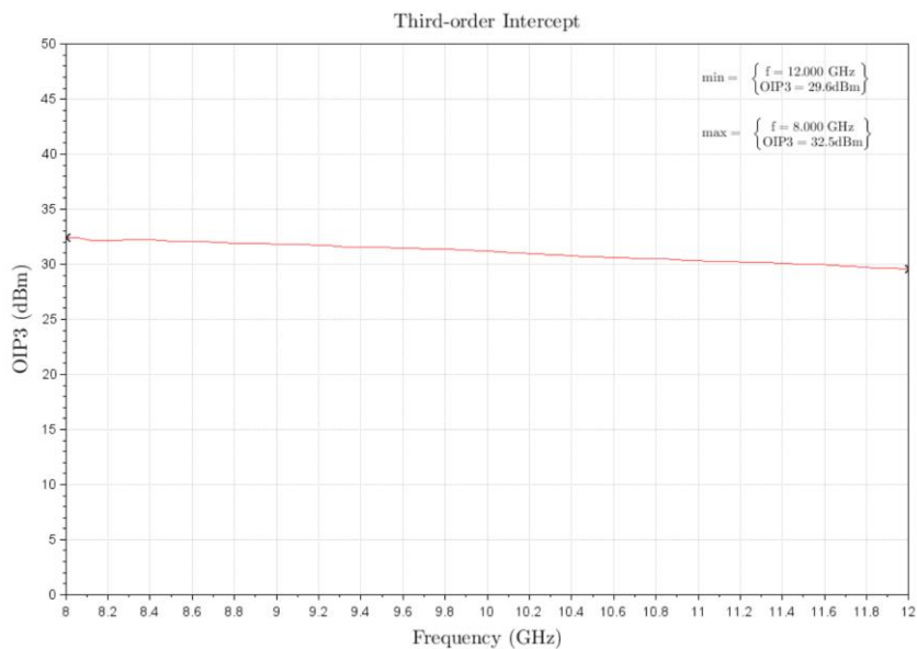
Figure 2: ERZ-LNA-0800-1200-10-6 OIP3
