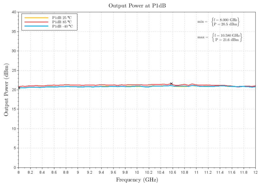
Figure 1: ERZ-LNA-0800-1200-10-6 P1dB
