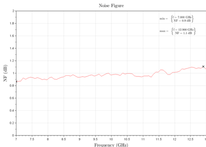
Figure 4: ERZ-LNA-0700-1300-51-1-NS Noise Figure
