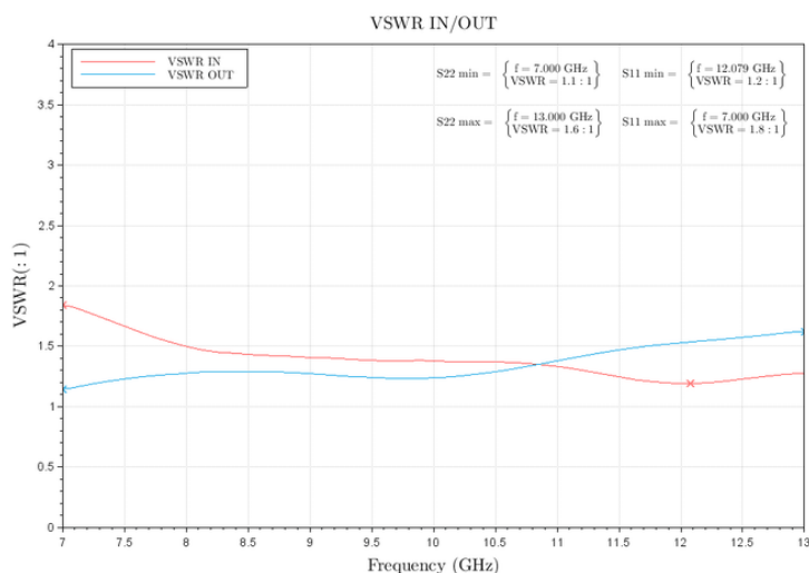
Figure 3: ERZ-LNA-0700-1300-51-1-NS Input&Output Matching
