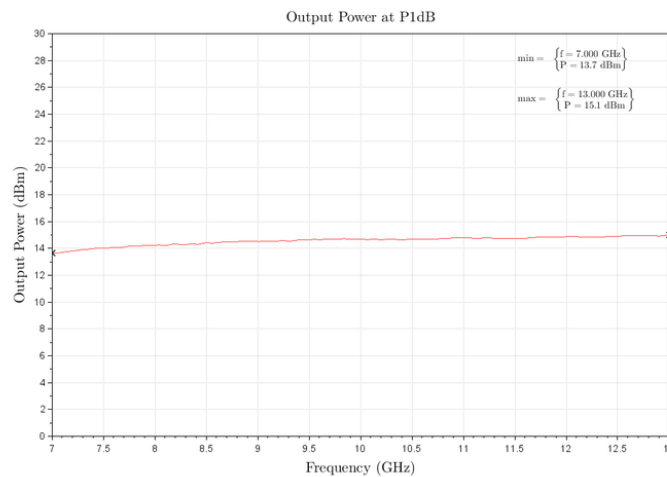
Figure 1: ERZ-LNA-0700-1300-51-1-NS P1dB
