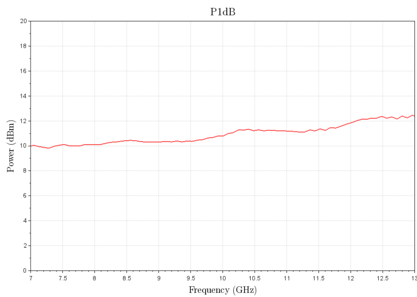
Figure 1: ERZ-LNA-0700-1300-21-1-NS P1dB
