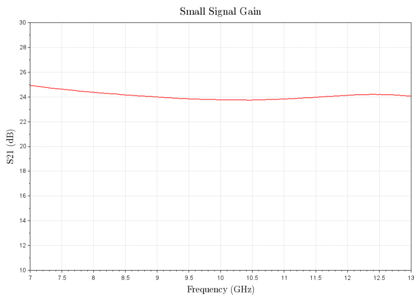
Figure 2: ERZ-LNA-0700-1300-21-1-NS Small Signal Gain
