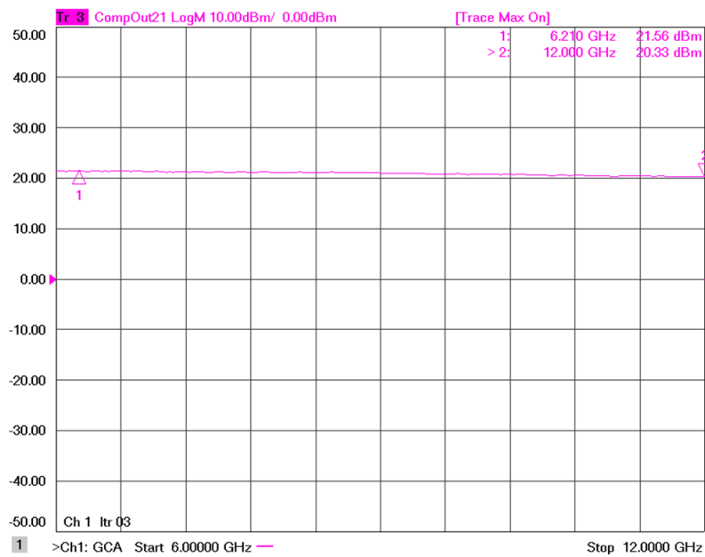
Figure 1: ERZ-LNA-0600-1200-35-3 P1dB
