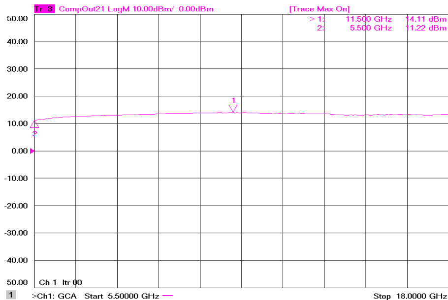
Figure 1: ERZ-LNA-0550-1800-40-4 P1dB
