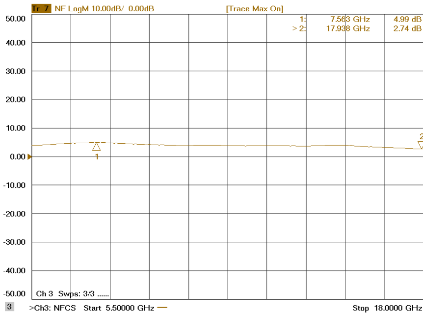
Figure 4: ERZ-LNA-0550-1800-40-4 Noise Figure
