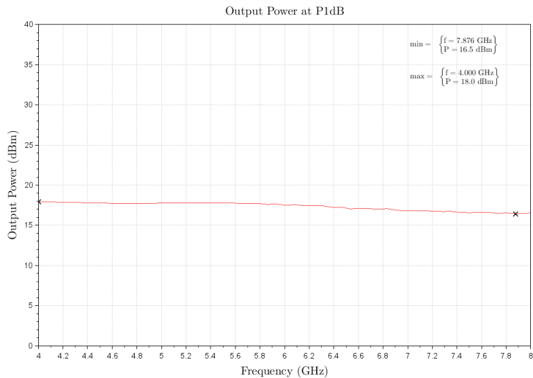
Figure 1: ERZ-LNA-0400-0800-28-1 P1dB
