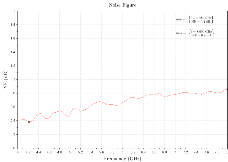
Figure 3: ERZ-LNA-0400-0800-28-1 Noise Figure
