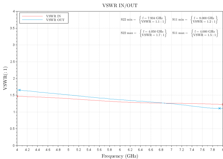
Figure 4: ERZ-LNA-0400-0800-28-1 Input and Output Matching
