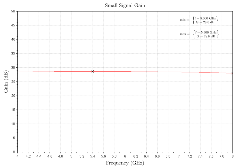
Figure 2: ERZ-LNA-0400-0800-28-1 Small Signal Gain
