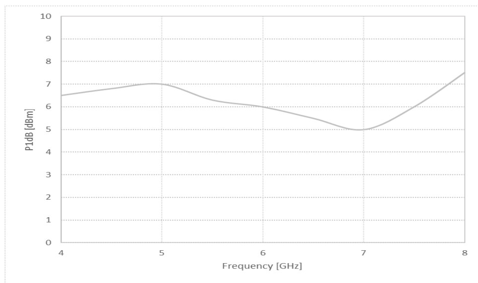
Figure 1: ERZ-LNA-0400-0800-28-1-NS P1dB
