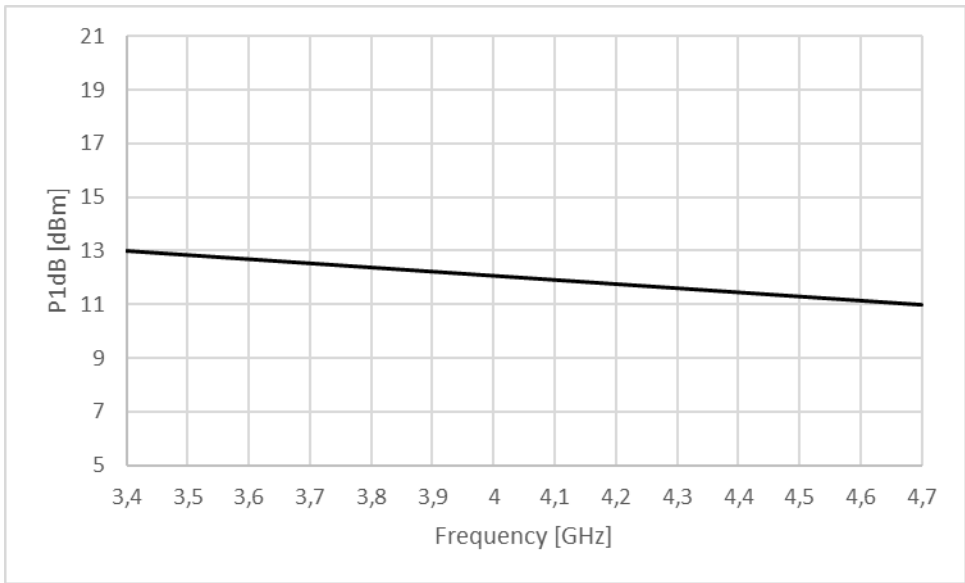
Figure 1: ERZ-LNA-0340-0470-23-2 P1dB
