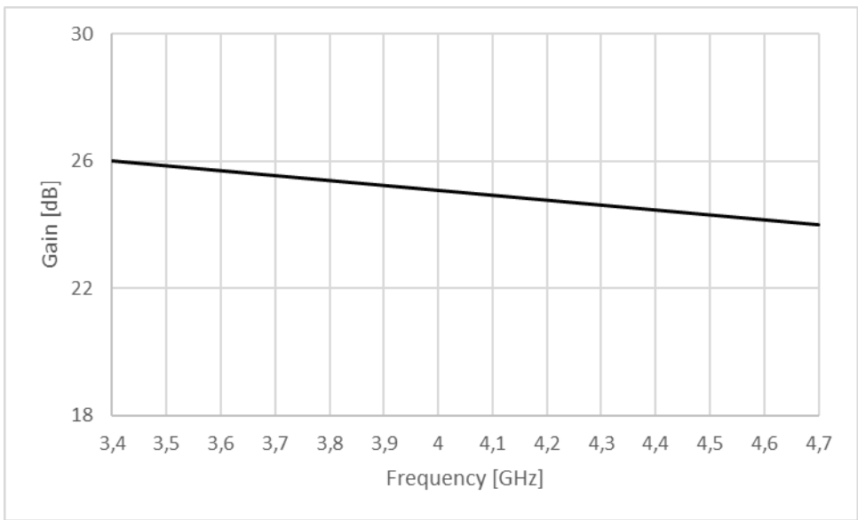
Figure 2: ERZ-LNA-0340-0470-23-2 Small Signal Gain
