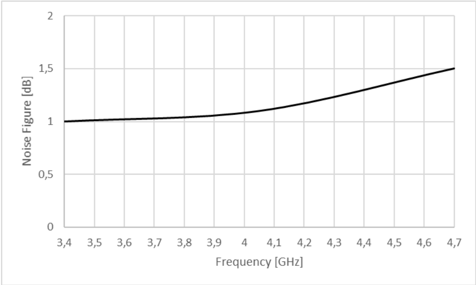
Figure 3: ERZ-LNA-0340-0470-23-2 Noise Figure
