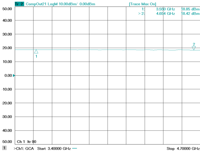
Figure 1: ERZ-LNA-0340-0470-13-2 P1dB
