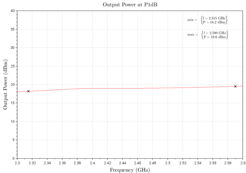
Figure 1: ERZ-LNA-0230-0260-40-2.5 P1dB
