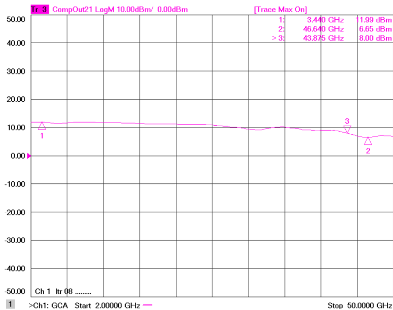
Figure 1: ERZ-LNA-0200-5000-22-6 P1dB
