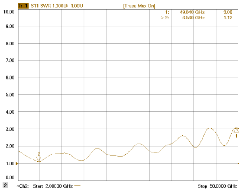
Figure 4: ERZ-LNA-0200-5000-22-6 Input Matching
