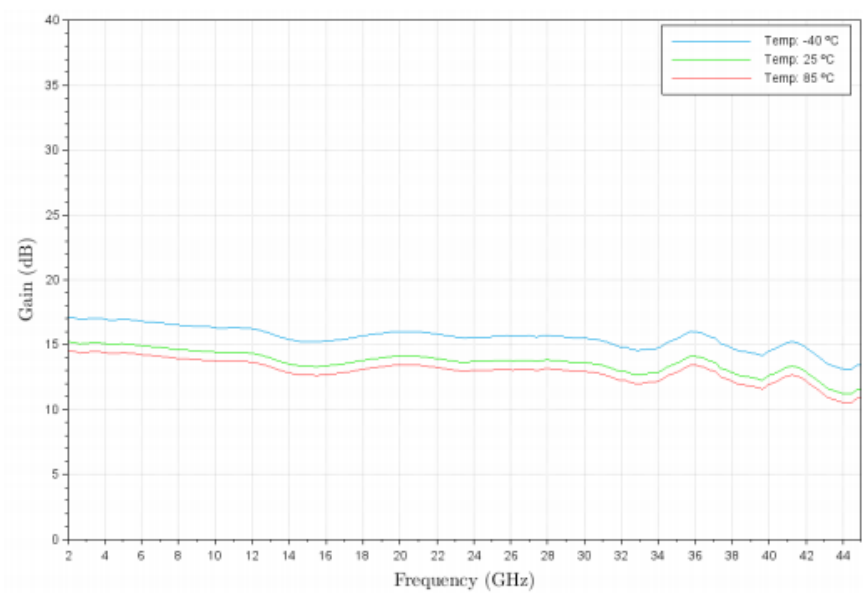
Figure 2: ERZ-LNA-0200-4500-15-4 Small Signal Gain
