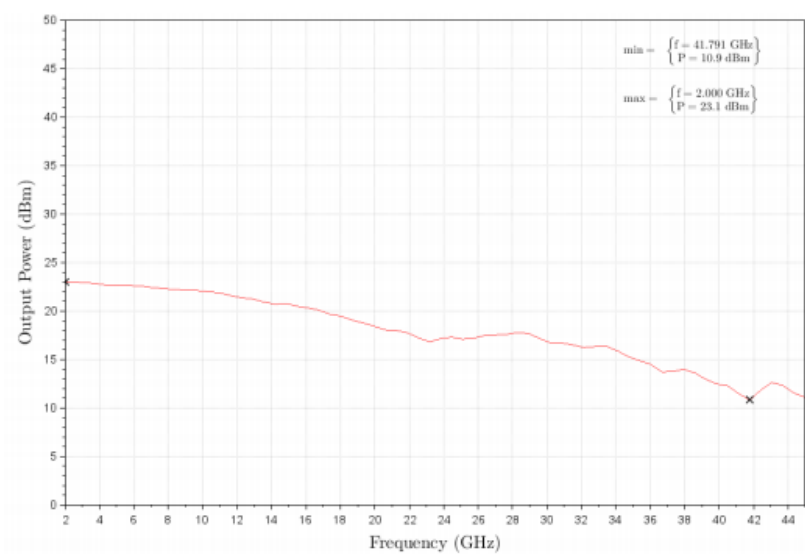
Figure 1: ERZ-LNA-0200-4500-15-4 P1dB
