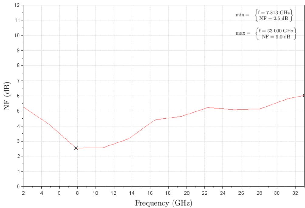
Figure 3: ERZ-LNA-0200-3300-30-4 Noise Figure
