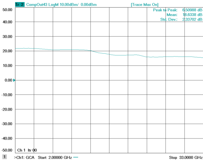
Figure 1: ERZ-LNA-0200-3300-30-4 P1dB
