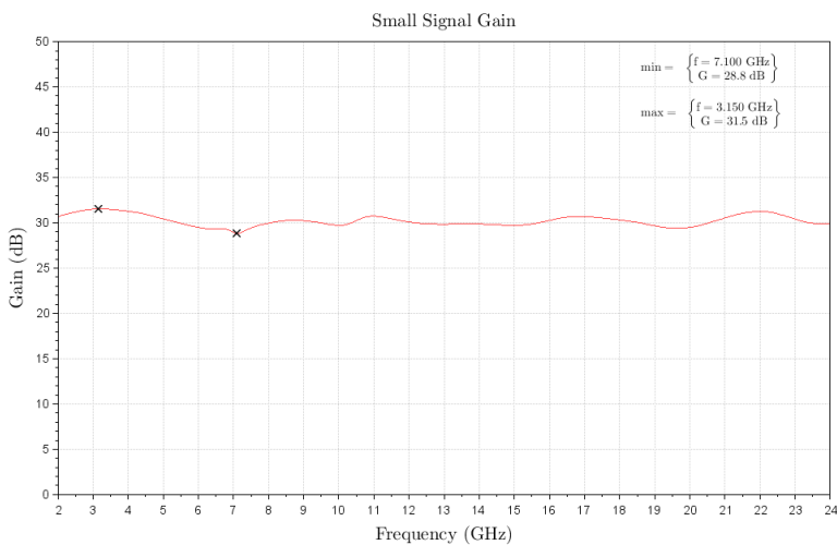
Figure 2: Figure 1: ERZ-LNA-0200-2400-30-3 Small Signal Gain
