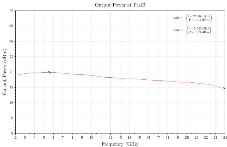
Figure 1: ERZ-LNA-0200-2400-30-3 Output Power at 1dB compression
