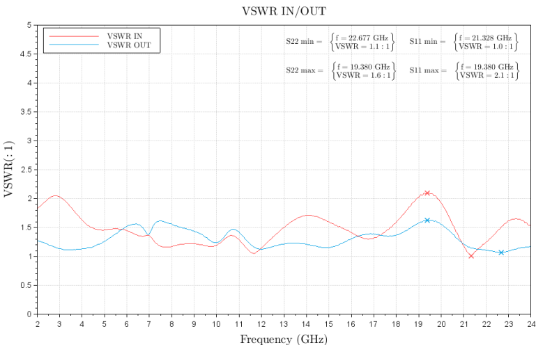
Figure 4: ERZ-LNA-0200-2400-15-3 Input and Output Matching
