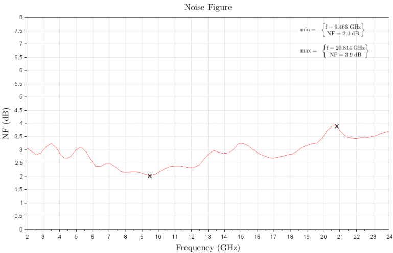
Figure 3: ERZ-LNA-0200-2400-30-3 Noise Figure
