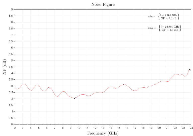
Figure 3: ERZ-LNA-0200-2400-15-3 Noise Figure
