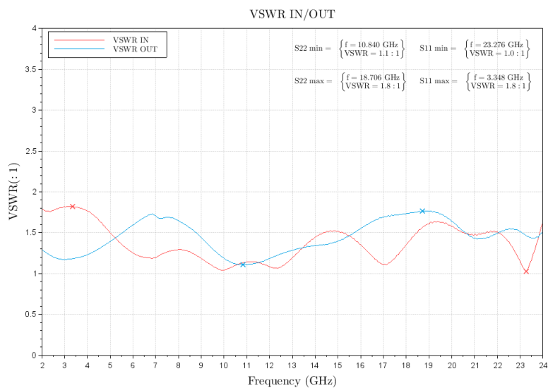
Figure 4: ERZ-LNA-0200-2400-15-3 Input and Output Matching
