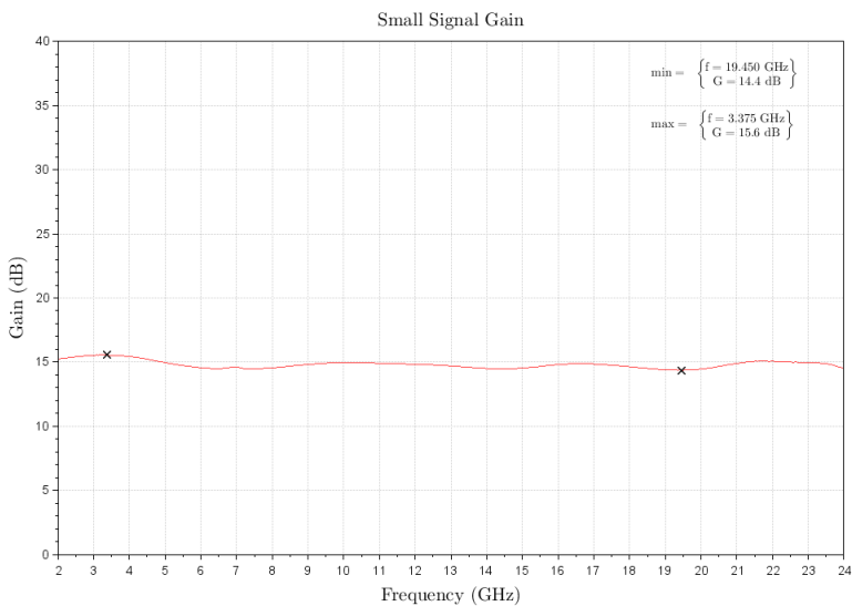
Figure 2: Figure 1: ERZ-LNA-0200-2400-15-3 Small Signal Gain
