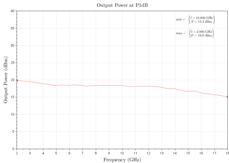
Figure 1-1: ERZ-LNA-0200-1800-30-2 P1dB
