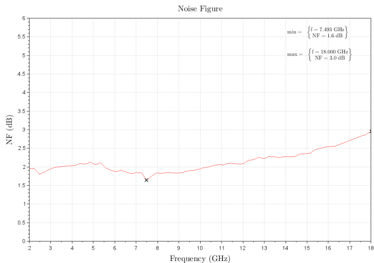
Figure 1-3: ERZ-LNA-0200-1800-30-2 Noise Figure
