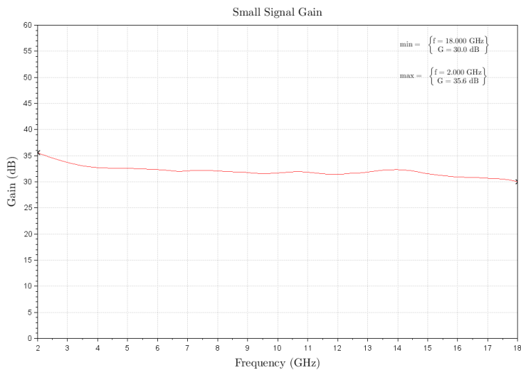
Figure 1-2: ERZ-LNA-0200-1800-30-2 Small Signal Gain
