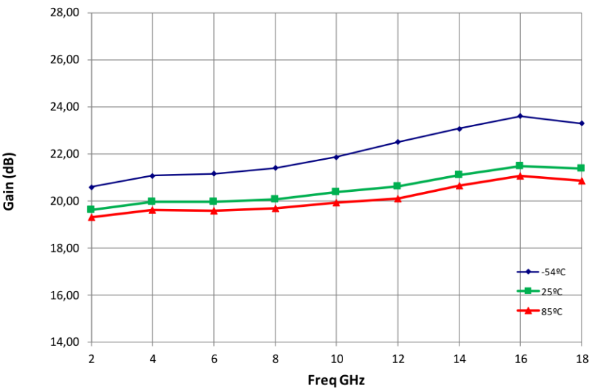
Figure 3: ERZ-LNA-0200-1800-18-4 Small Signal Gain Vs Temperature
