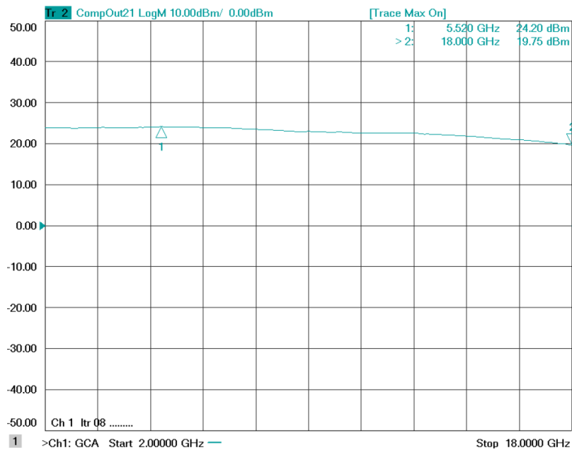
Figure 1: ERZ-LNA-0200-1800-18-4 P1dB
