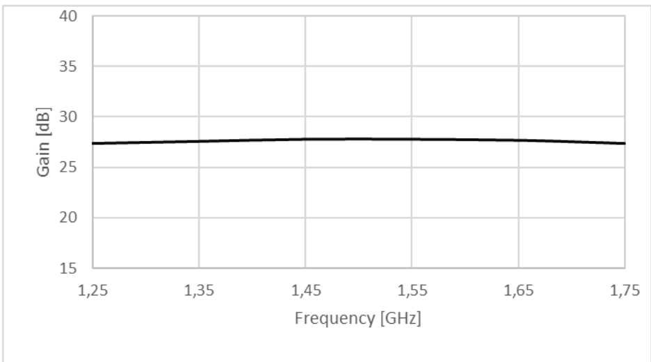
Figure 2: ERZ-LNA-0125-0175-27-2 Small Signal Gain
