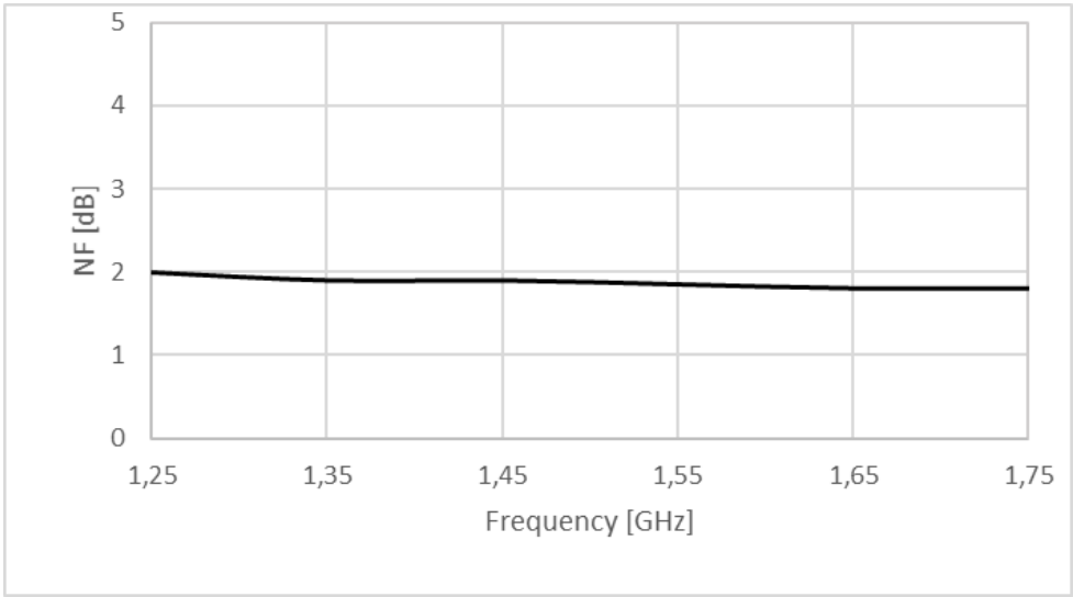
Figure 3: ERZ-LNA-0125-0175-27-2 Noise Figure
