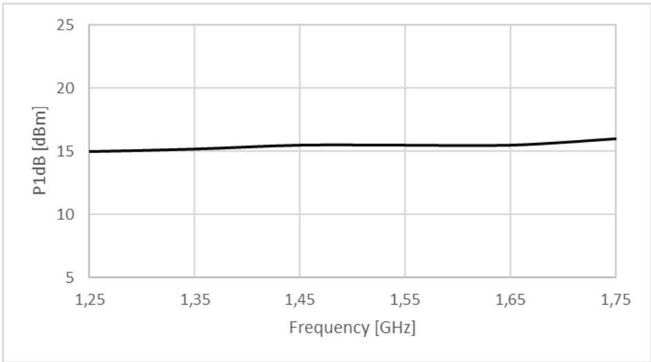
Figure 1: ERZ-LNA-0125-0175-27-2 P1dB
