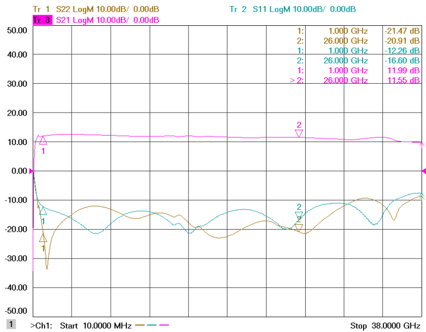
Figure 1: ERZ-LNA-0100-3800-12-4 S-parameters
