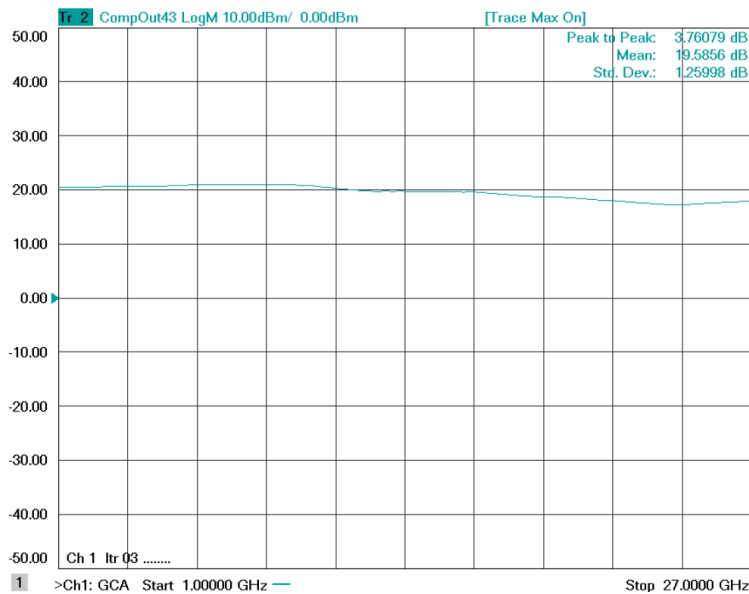
Figure 1: ERZ-LNA-0100-2700-45-4 P1dB
