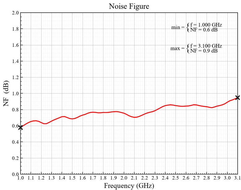
Figure 1-3: ERZ-LNA-0100-0310-32-0.9 Noise Figure
