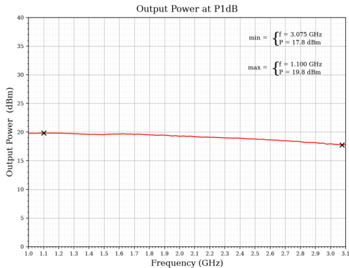
Figure 1-1: ERZ-LNA-0100-0310-32-0.9 P1dB
