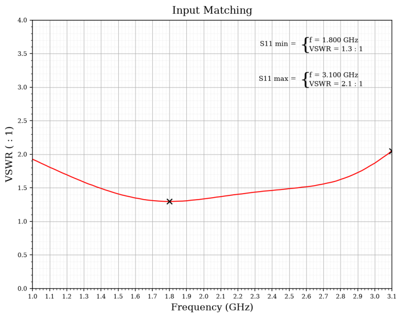
Figure 1-4: ERZ-LNA-0100-0310-32-0.9 Input Matching
