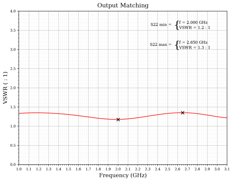
Figure 1-5: ERZ-LNA-0100-0310-32-0.9 Output Matching
