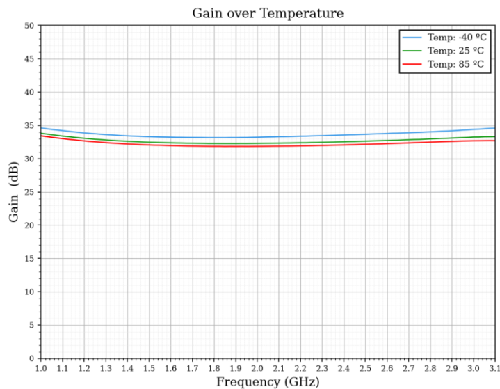
Figure 1-2: ERZ-LNA-0100-0310-32-0.9 Small Signal Gain
