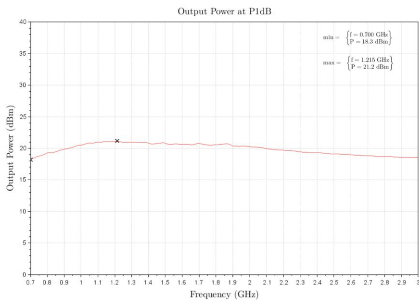
Figure 1: ERZ-LNA-0070-0300-20-0.7-NS P1dB
