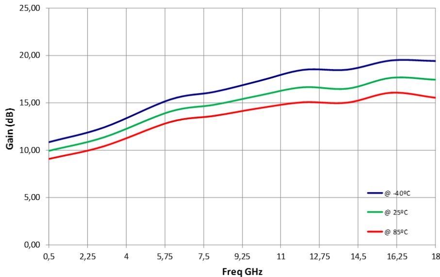
Figure 2: ERZ-LNA-0050-1800-15-3 Small Signal Gain Vs Temperature
