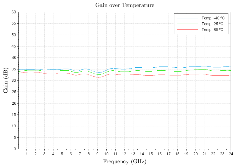
Figure 3: ERZ-LNA-0010-2400-30-4 Gain over Temperature
