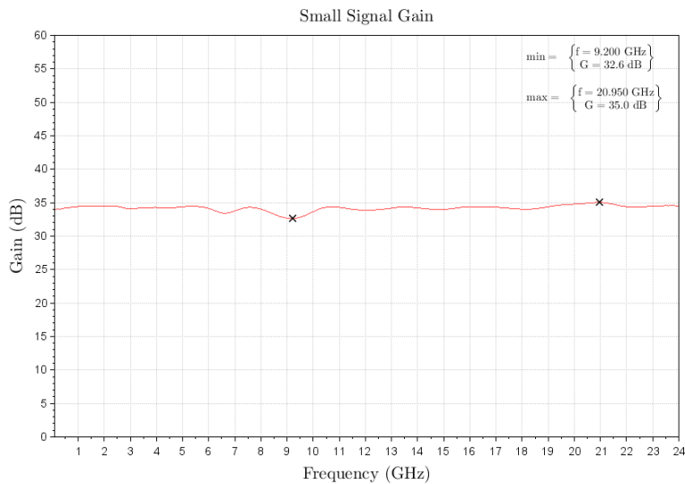
Figure 2: ERZ-LNA-0010-2400-30-4 Small Signal Gain
