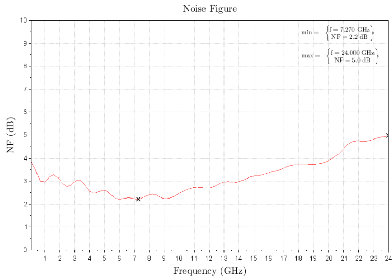
Figure 4: ERZ-LNA-0010-2400-30-4 Noise Figure
