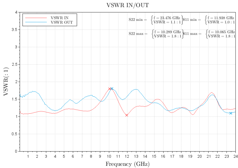
Figure 5: ERZ-LNA-0010-2400-30-4 Input & Output Matching
