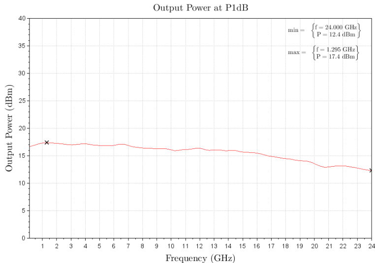
Figure 1: ERZ-LNA-0010-2400-30-4 P1dB
