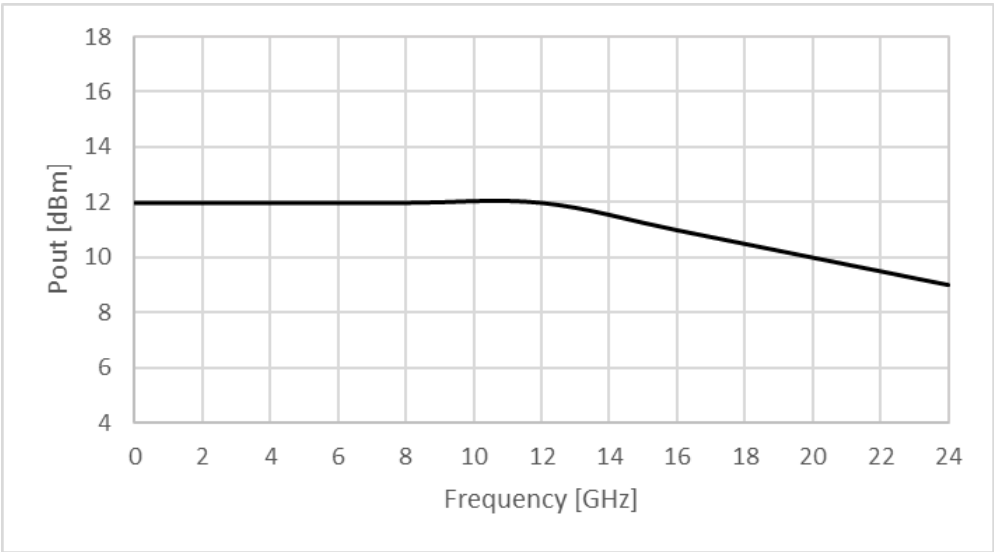
Figure 1: ERZ-LNA-0010-2400-14-4 P1dB
