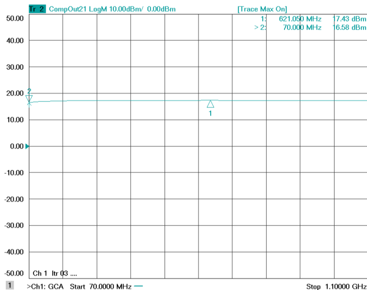
Figure 1-1: ERZ-LNA-0007-0110-28-2 P1dB
