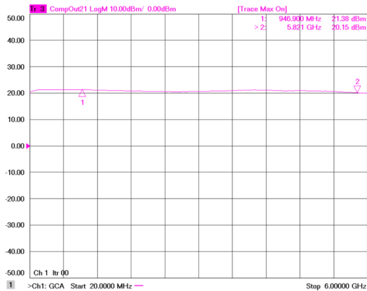
Figure 1: ERZ-LNA-0002-0600-30-2 P1dB
