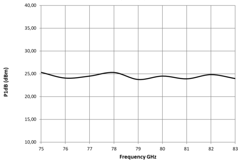
Figure 1: ERZ-HPA-7500-8300-27 P1dB
