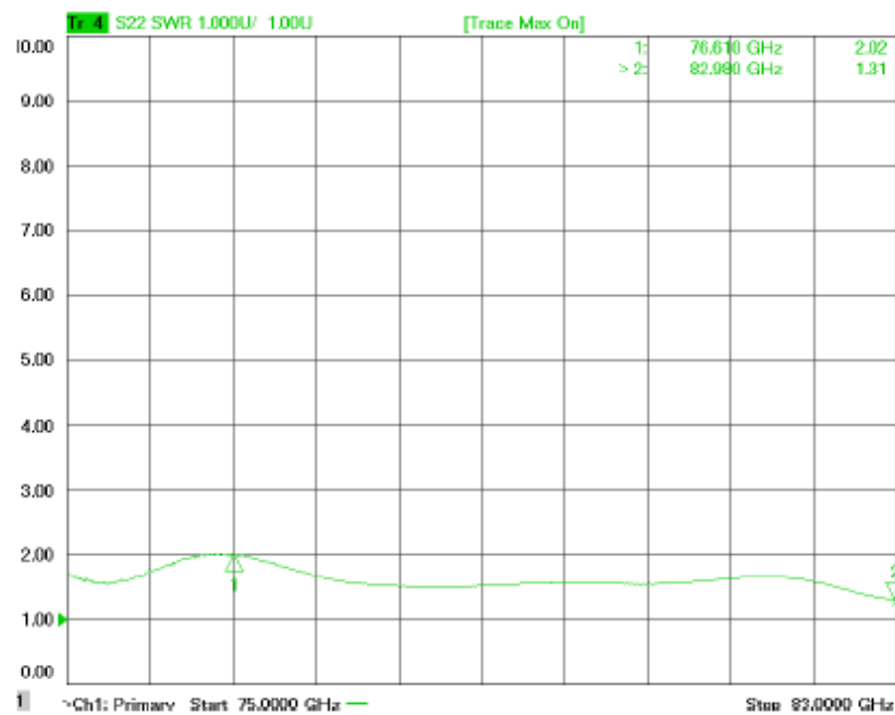
Figure 4: ERZ-HPA-7500-8300-27 Output Matching
