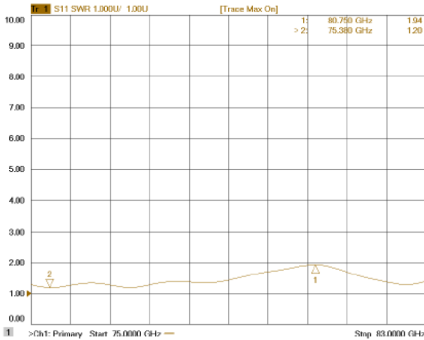
Figure 3: ERZ-HPA-7500-8300-27 Input Matching
