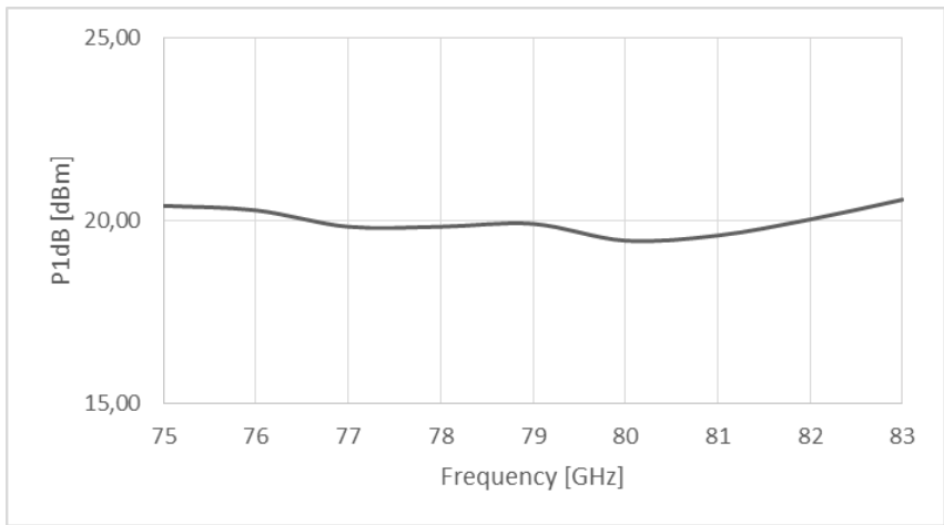
Figure 1: ERZ-HPA-7500-8300-25 P1dB
