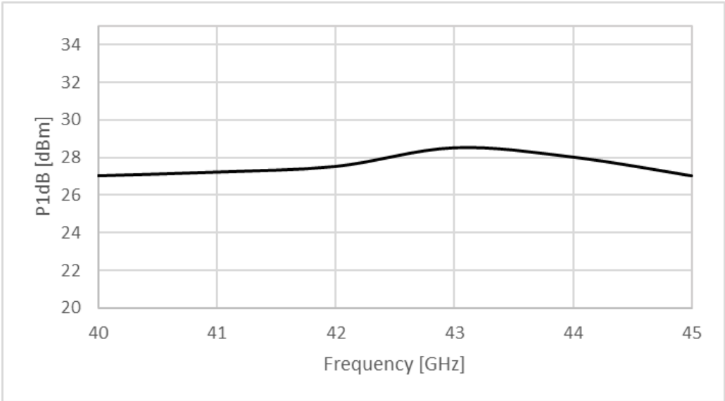
Figure 1: ERZ-HPA-4000-4500-28-E P1dB
