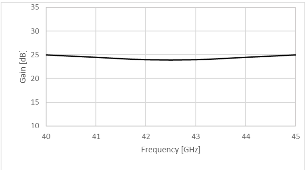
Figure 2: ERZ-HPA-4000-4500-28-E Small Signal Gain
