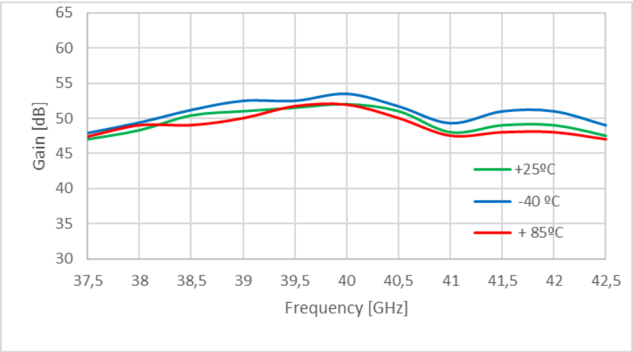
Figure 2: ERZ-HPA-3750-4250-39 Gain
