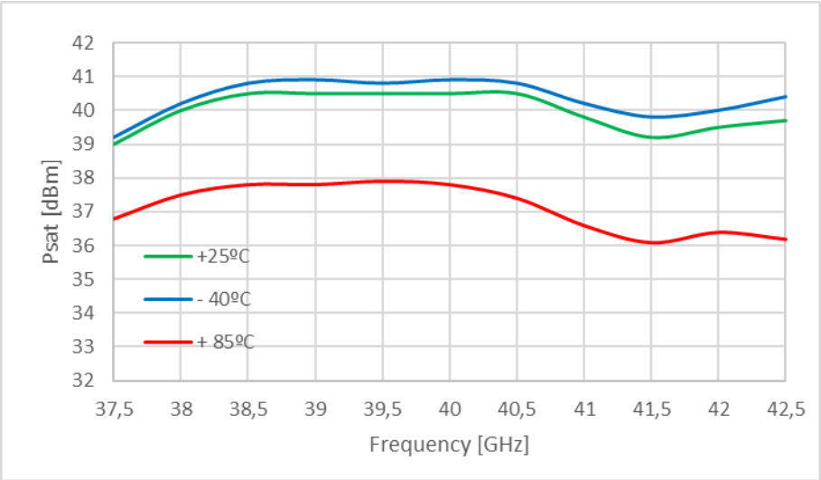
Figure 1: ERZ-HPA-3750-4250-39 Psat
