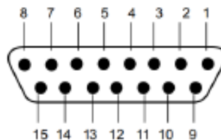
Figure 3-1: M83513/02-BN (female).
