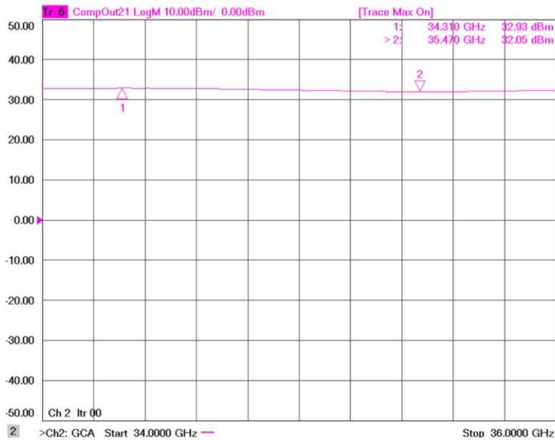
Figure 1: ERZ-HPA-3400-3600-33 Psat
