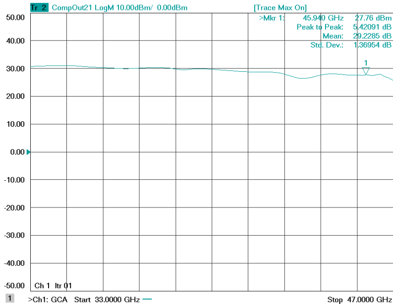
Figure 1: ERZ-HPA-3300-4700-29 Psat
