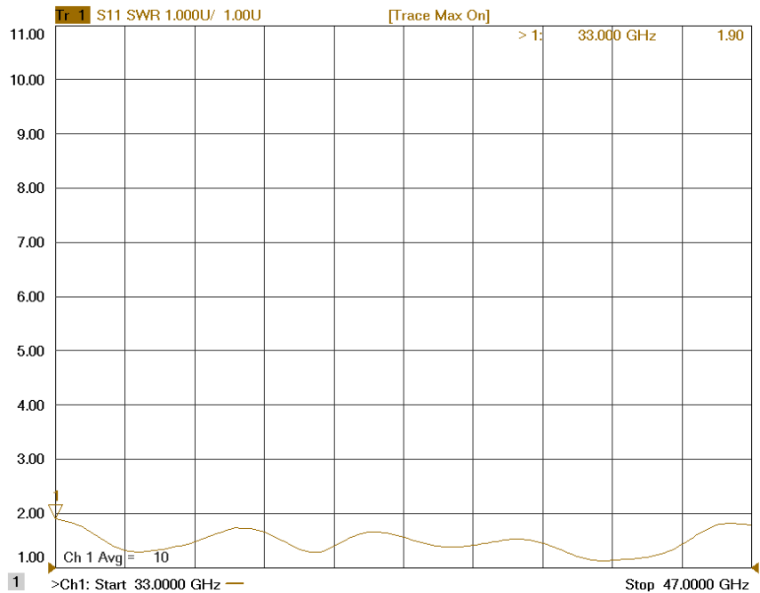
Figure 4: ERZ-HPA-3300-4700-24-E Input Matching
