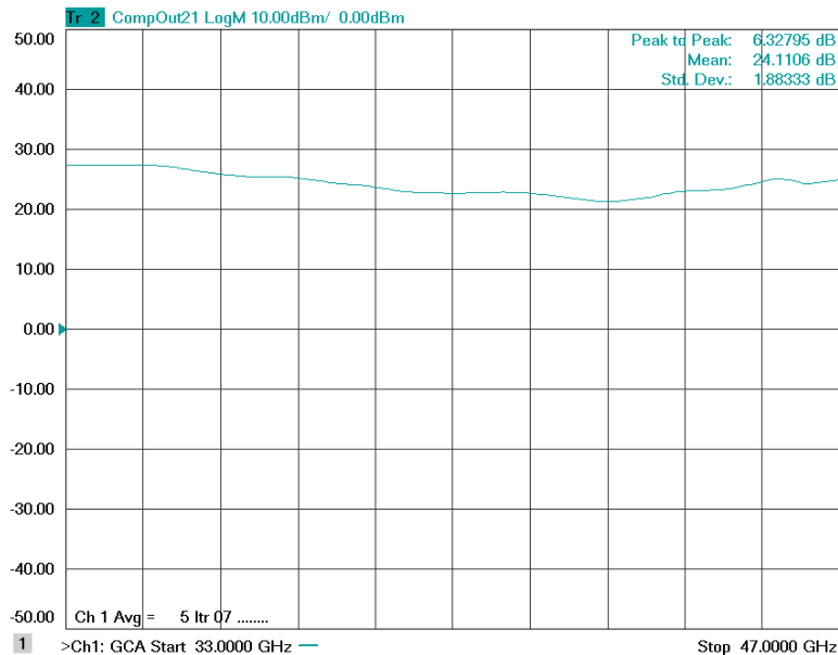
Figure 1: ERZ-HPA-3300-4700-24-E Psat
