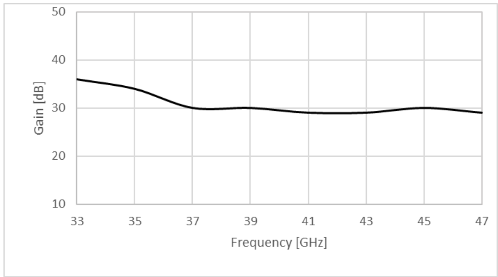
Figure 2: ERZ-HPA-3300-4700-24-E Small Signal Gain
