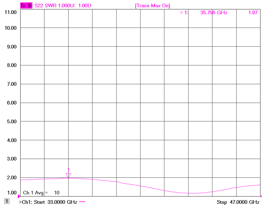
Figure 5: ERZ-HPA-3300-4700-24-E Output Matching
